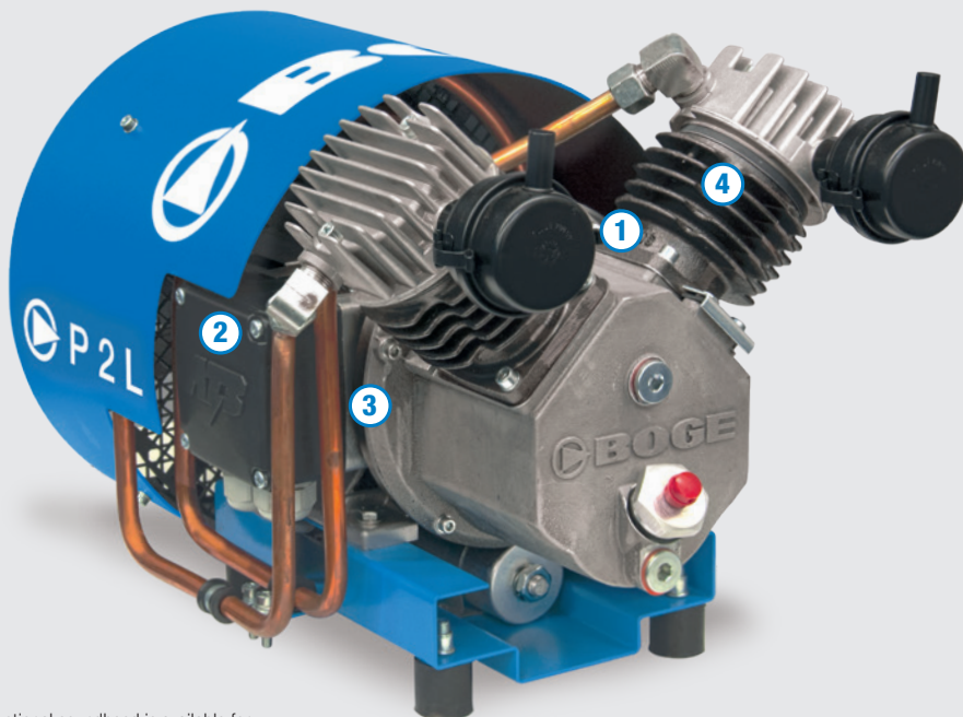
An optional soundhood is available for models P 1 L and P 2 L to further reduce noise levels.
